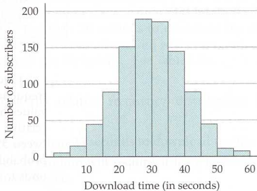
Figure 12.3 A histogram for the frequency distribution in Table 12.4
