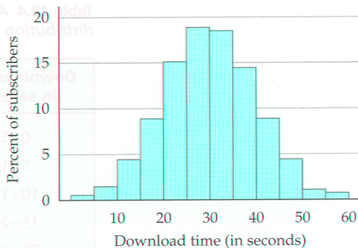
Figure 12.4 A relative frequency histogram
